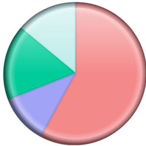
Dwelling Type - Scarborough 4020
